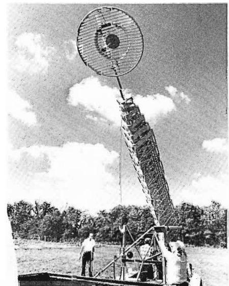
Telescoping 100 foot tower carried on separate trailer is used for remote microwave transmission.
