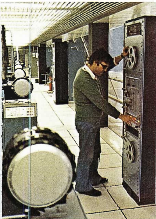
PM-86SL Magnetic Reproducers provide Sep-sound facilities for the telecine operation.
