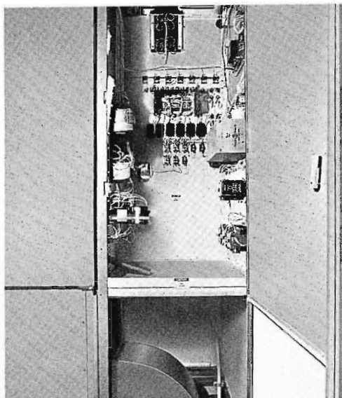
The blower was removed from the transmitter and located in a "clean air" room in the basement, with the output ducted to the bottom of transmitter for cool, quiet operation.
