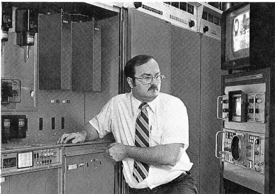
Director of Engineering John Bosak checks set-up adjustments for Mod Anode Pulser. Transmitter operating power cost savings with the pulser have been measured at $1.58 per hour by WITF.
