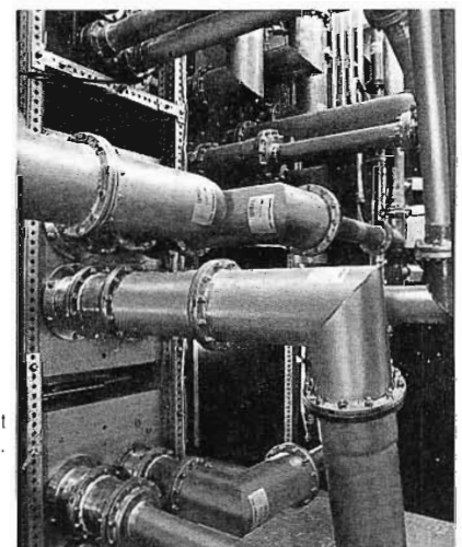
Transfer panel at WITF-TV. Manual patch panel at left; motorized coaxial switches on right.
