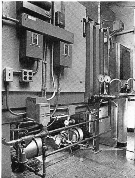
Compact heat exchanger for TTU-60 is raised off the floor to permit access to water storage pumps beneath.
